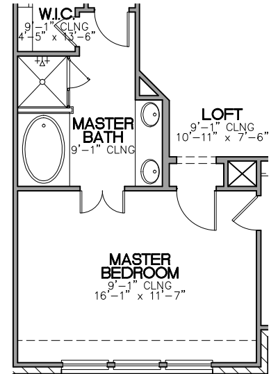
* Master Bath Option Second Floor Plan
