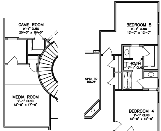
* Media Room Option Second Floor Plan
