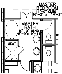
* Mud Shower Pan Option First Floor Plan
