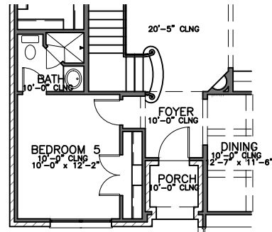
* Bedroom 5 ILO Study Option First Floor Plan
