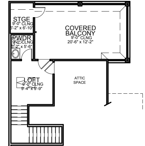
* Loft W/Balcony Option Third Floor Plan
