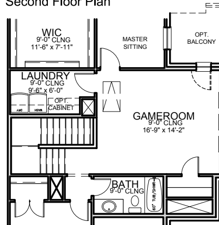
* Game Room Option (not available with 3rd floor opt.) Second Floor Plan
