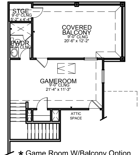
* Game Room W/Balcony Option Third Floor Plan
