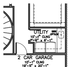
Utility Cabinet Option *First Floor Plan
