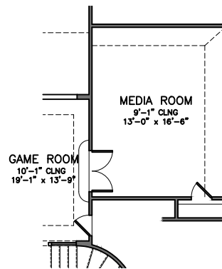
Media Room Option *2nd. Floor Plan
