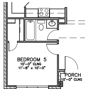
* Bedroom 5 Option First Floor Plan
