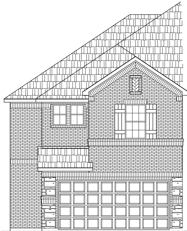
Elevation C
