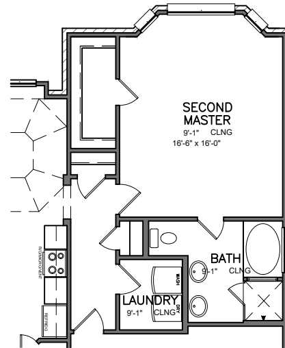
* Second Master Option First Floor Plan
