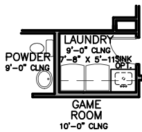
* Utility Cabinet Option Second Floor Plan
