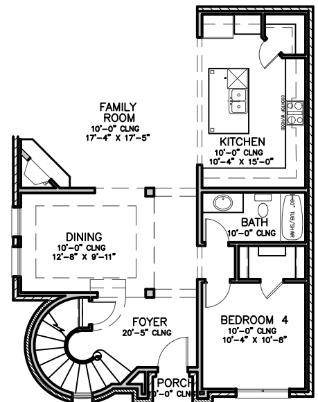
* Bedroom 4 Opt First Floor
