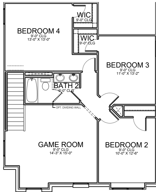
Second Floor
