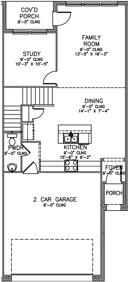
First Floor Plan INTERIOR UNIT
