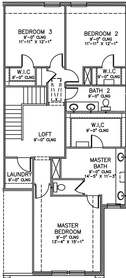
Second Floor Plan INTERIOR UNIT
