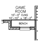
* Built-in Bench Option Second Floor Plan
