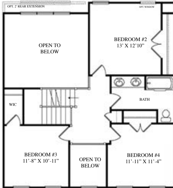
Second Floor - Elevation 1
