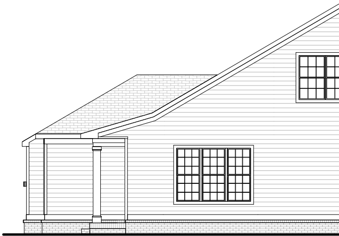
LEFT ELEVATION
