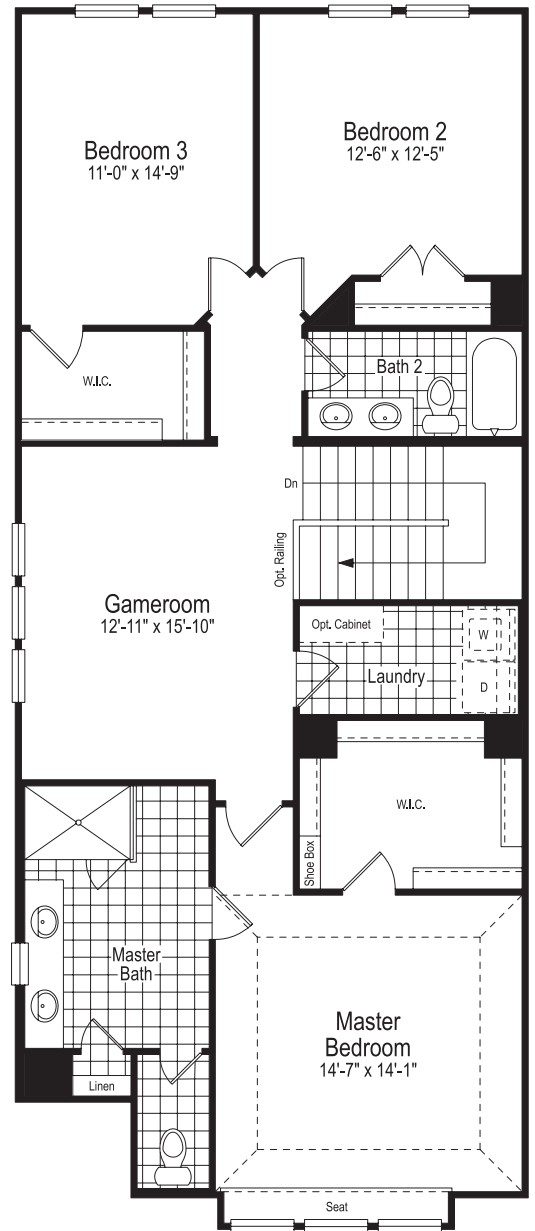
Second Floor
