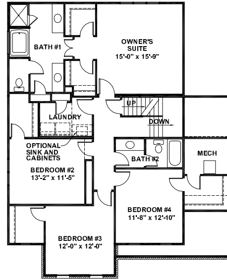
STANDARD SECOND FLOOR PLAN
