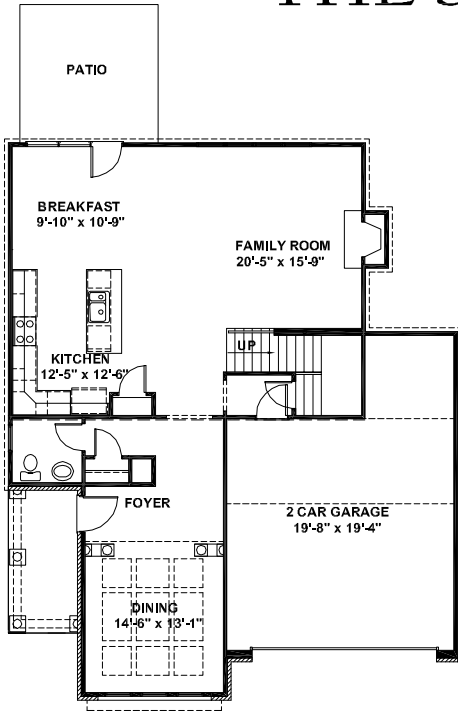
STANDARD FIRST FLOOR PLAN
