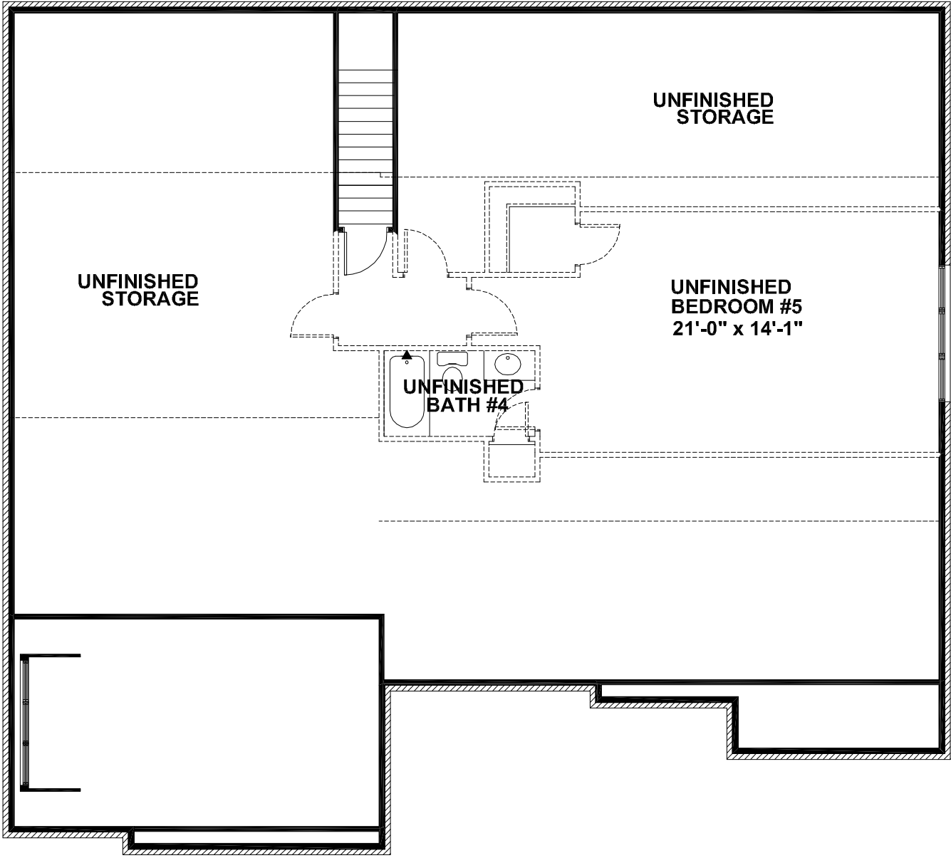
OPTIONAL ATTIC PLAN
