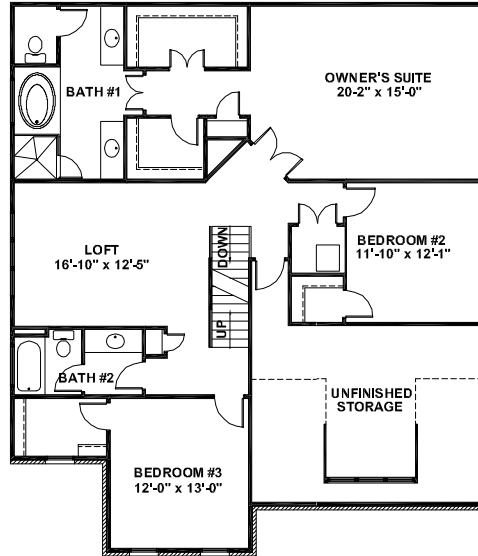
STANDARD SECOND FLOOR PLAN
