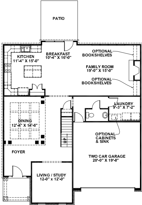
STANDARD FIRST FLOOR PLAN
