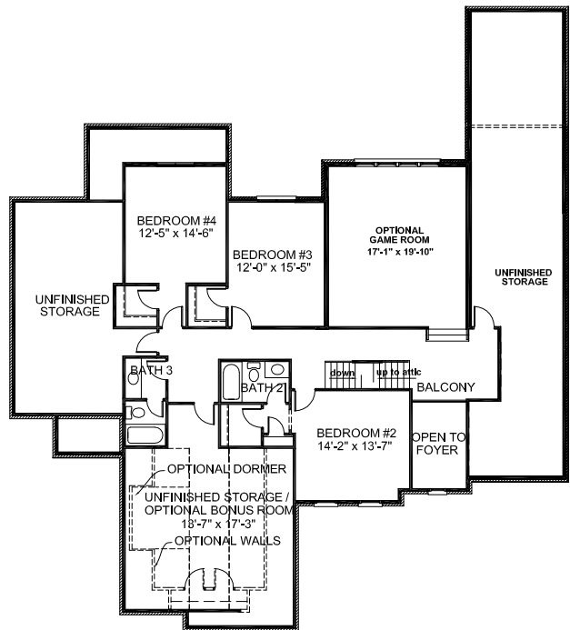
OPTIONAL SECOND FLOOR PLAN
