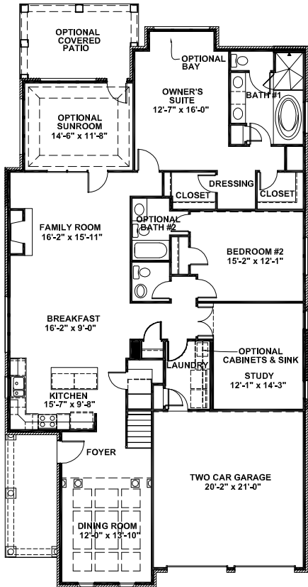
OPTIONAL FIRST FLOOR PLAN
