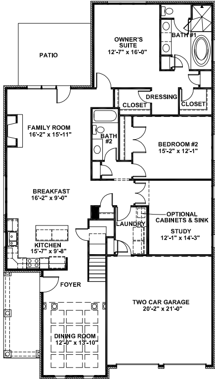
STANDARD FIRST FLOOR PLAN
