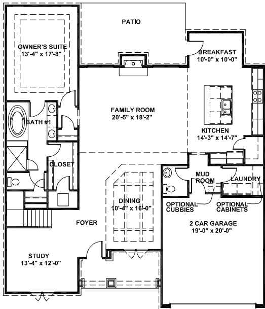
STANDARD FIRST FLOOR PLAN
