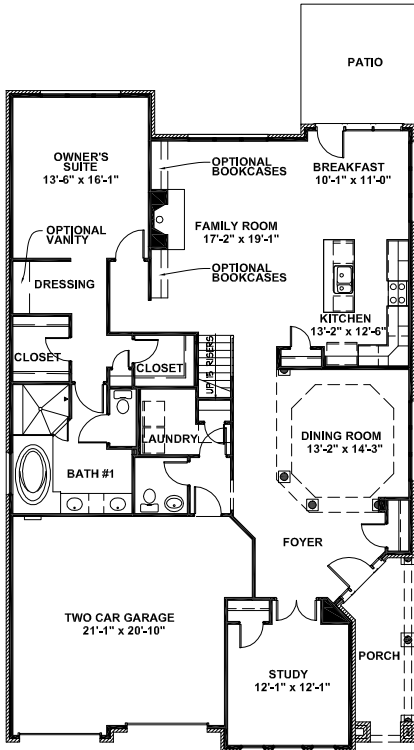
STANDARD FIRST FLOOR PLAN
