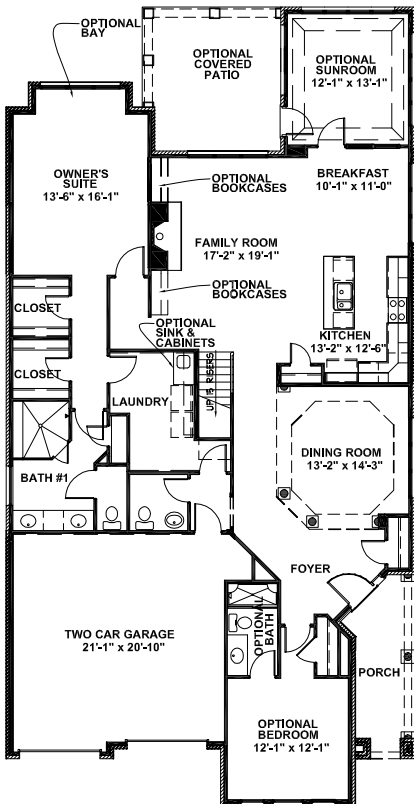
OPTIONAL FIRST FLOOR PLAN
