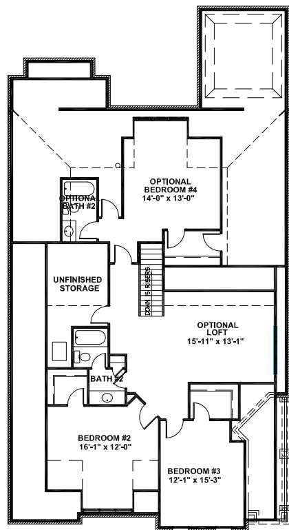
OPTIONAL SECOND FLOOR PLAN
