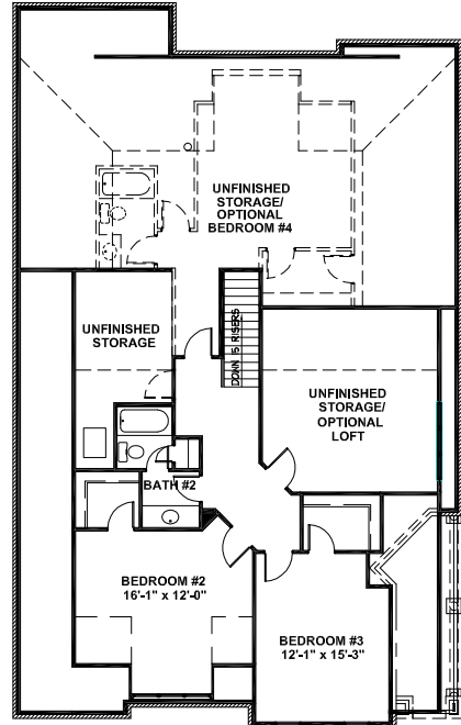
STANDARD SECOND FLOOR PLAN
