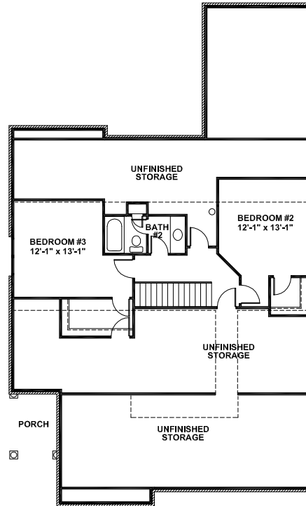
STANDARD SECOND FLOOR PLAN
