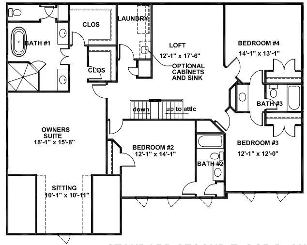
STANDARD SECOND FLOOR PLAN
