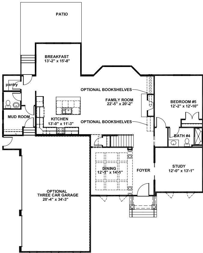
OPTIONAL FIRST FLOOR PLAN
