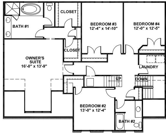
STANDARD SECOND FLOOR PLAN
