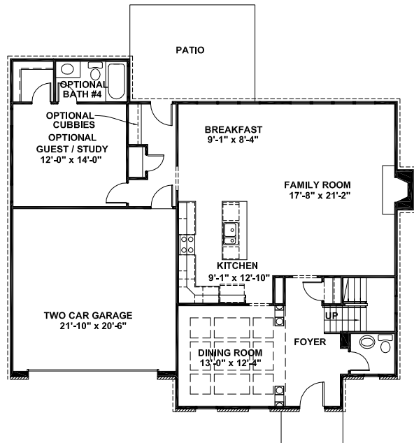
OPTIONAL FIRST FLOOR PLAN
