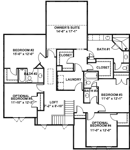
OPTIONAL SECOND FLOOR PLAN
