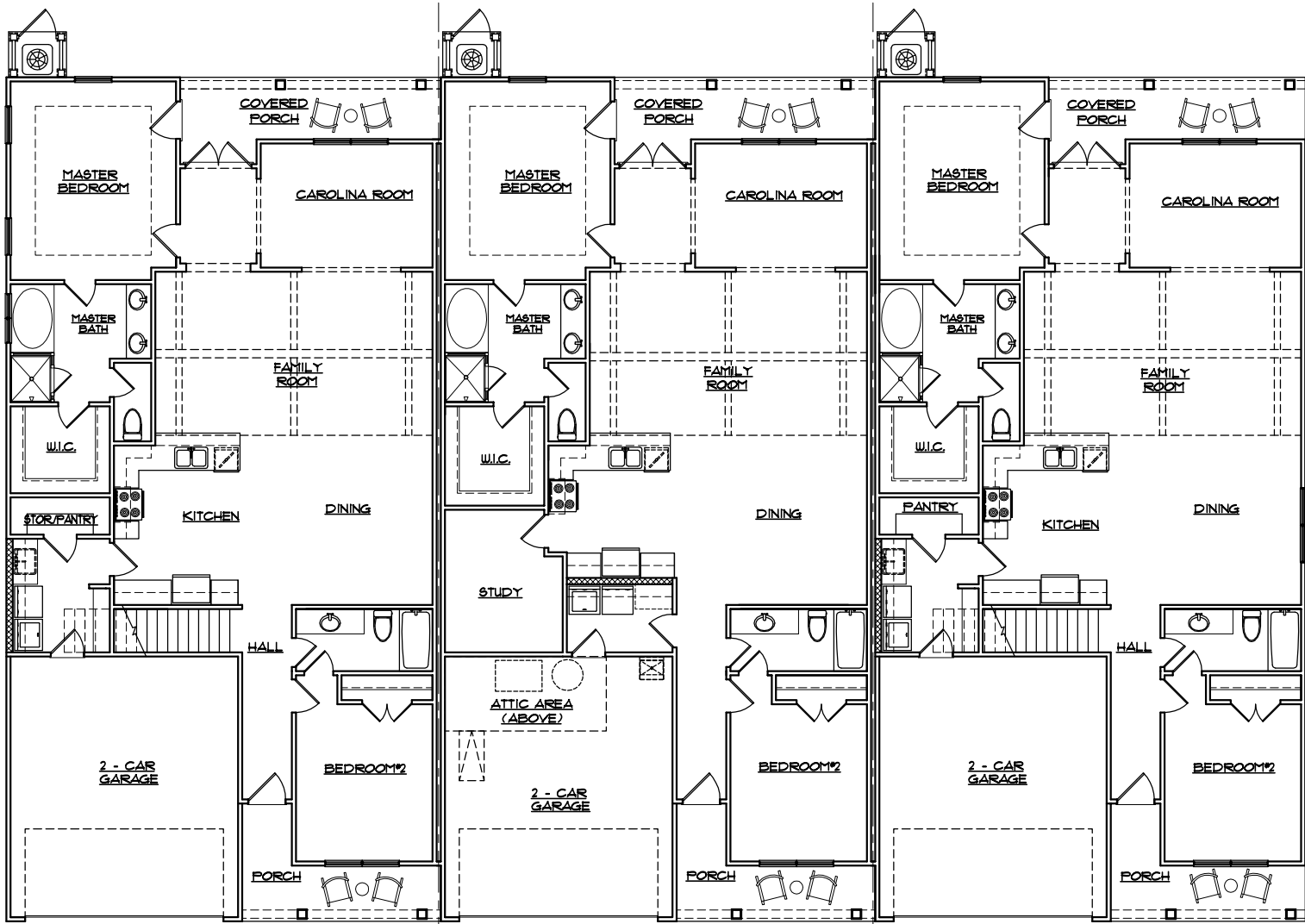
FIRST FLOOR PLAN - LOT 20 120 DANBURY COURT
