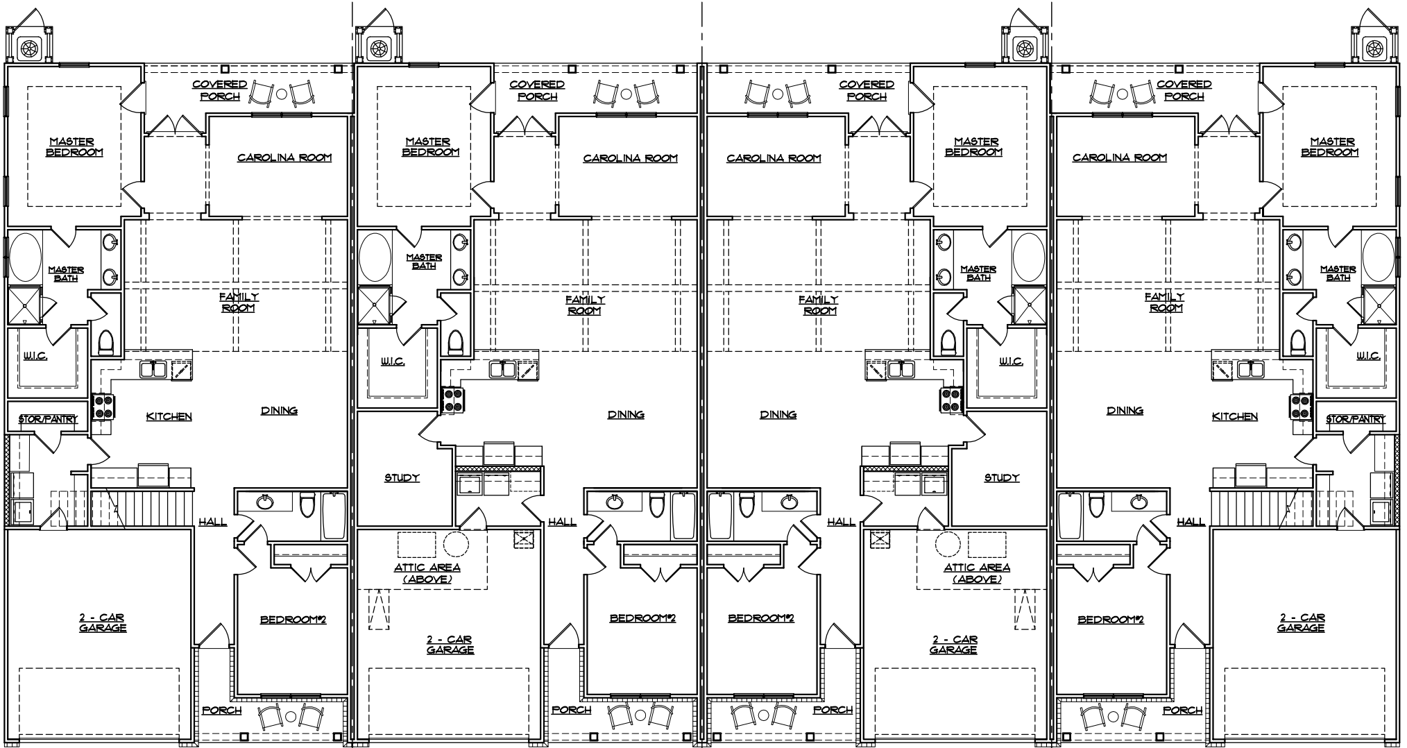
FIRST FLOOR PLAN - LOT 21 119 DANBURY COURT
