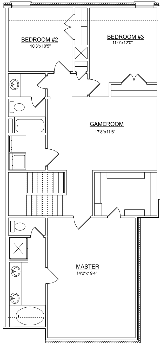
2nd Floor
