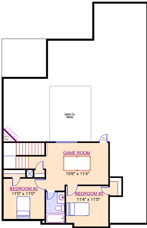
2nd Floor
