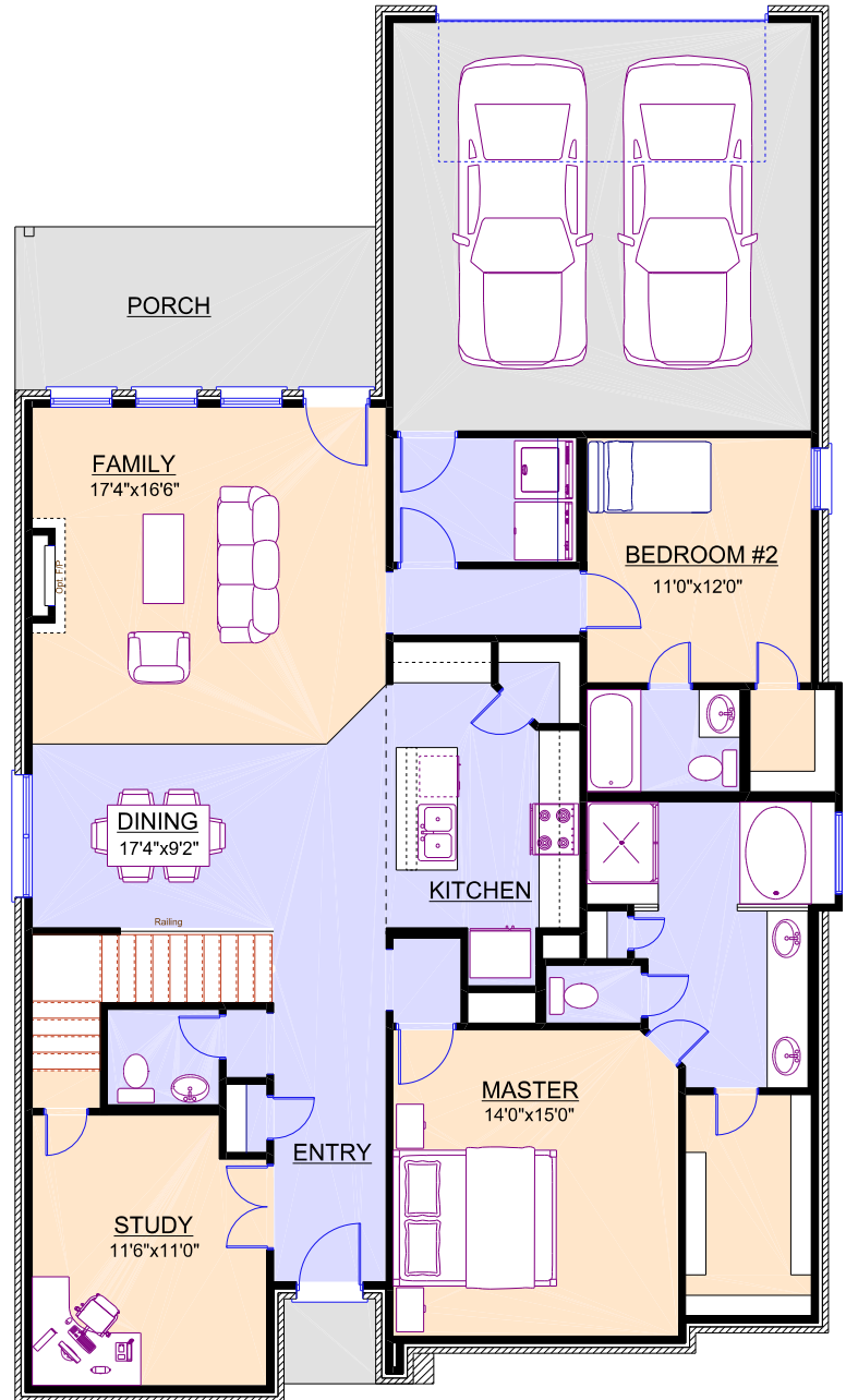
1st Floor
