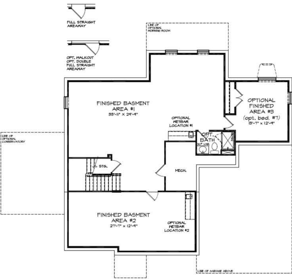
FINISHED (OPT.) BASEMENT FLOOR PLAN
